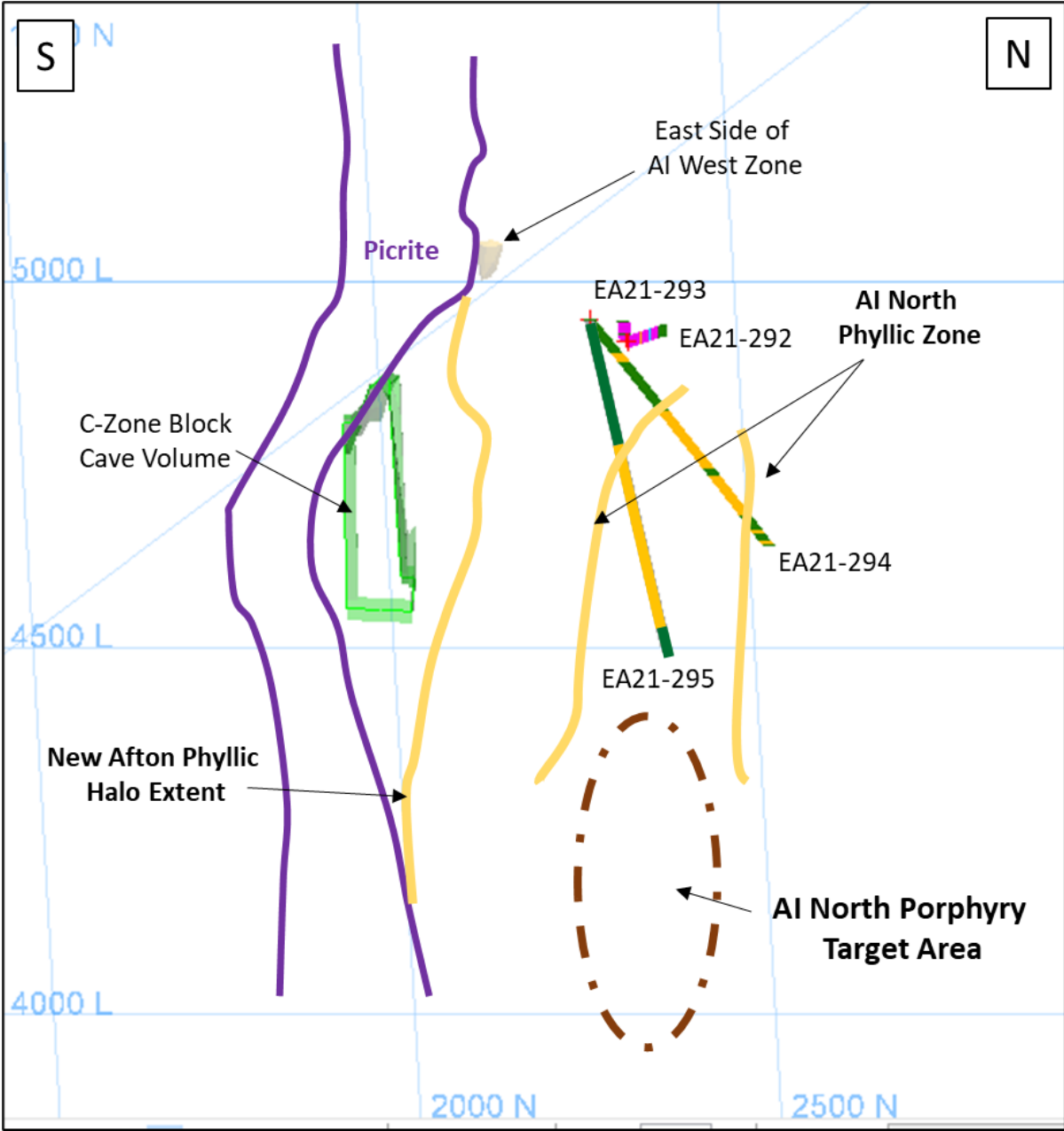
Figure 4: Cross section looking west showing interpreted alteration pattern within the AI North target area and potential location for porphyry style mineralization.
