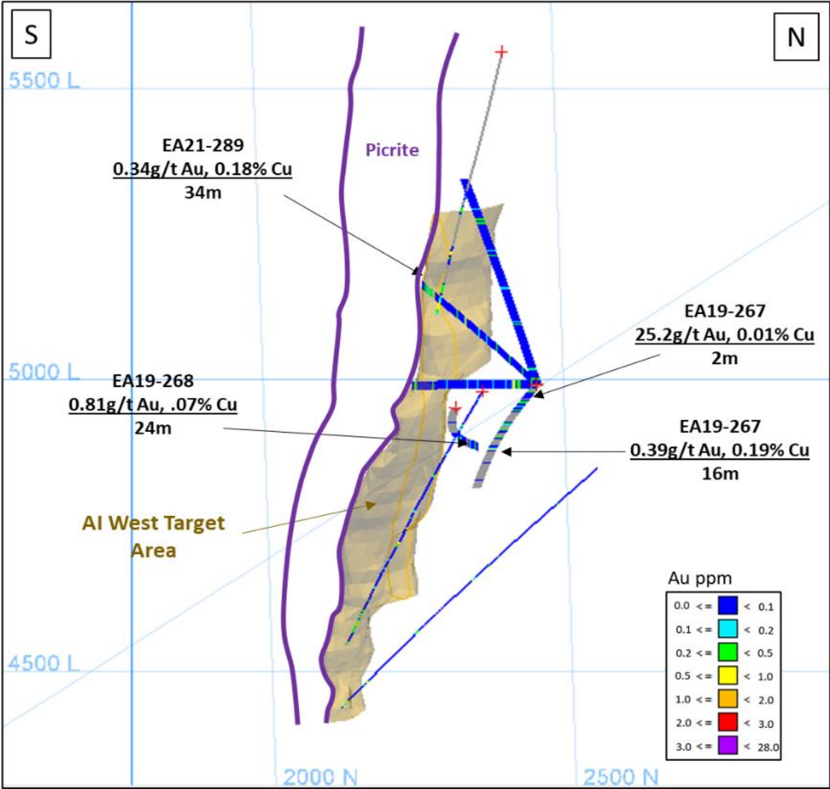
Figure 3: Cross section looking west showing interpreted AI West target area and assay results highlights on drill holes traces (EA21 exploration holes and EA19 geotechnical holes).
