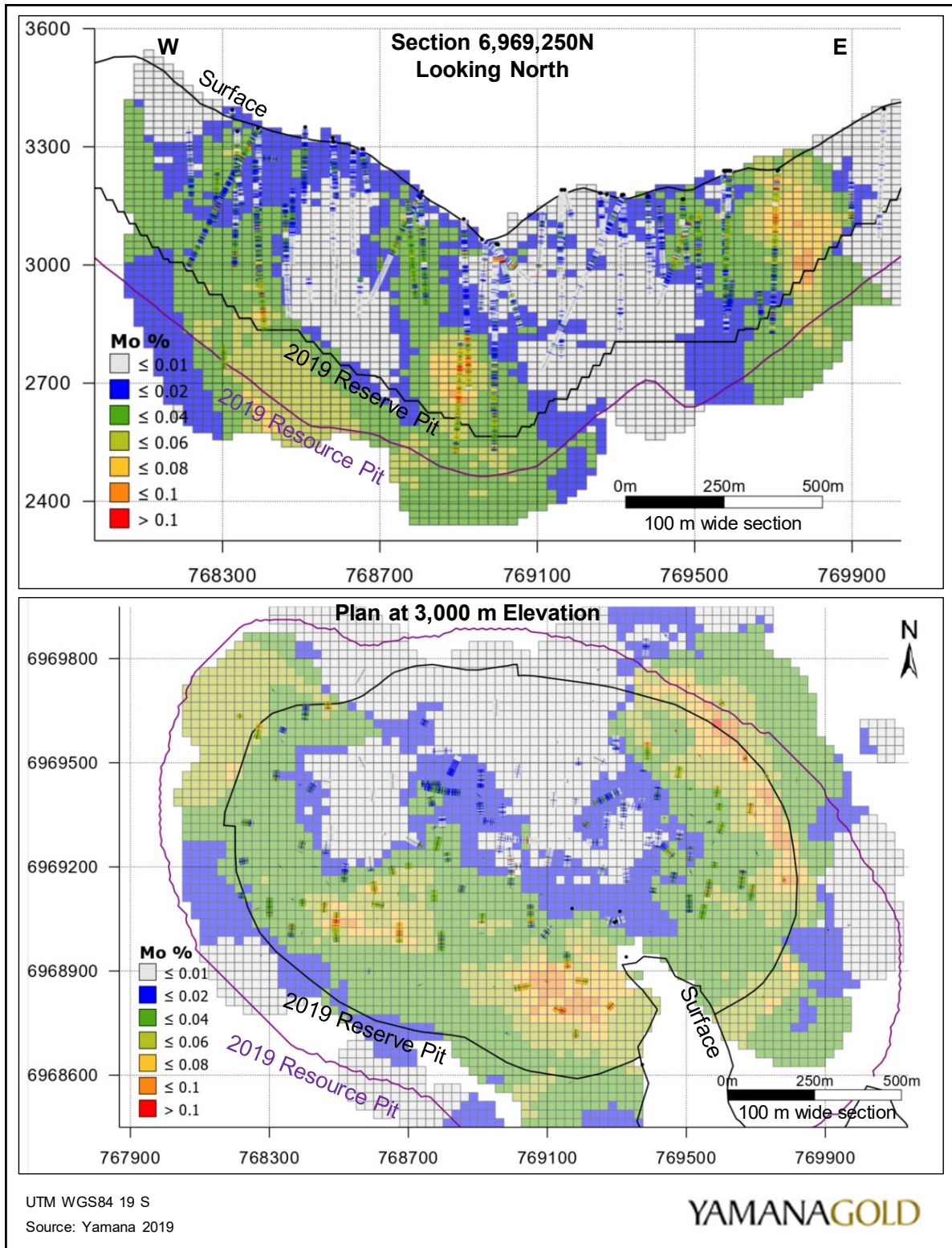
Figure 14-31: Estimated Molybdenum in Block Model and Drilling – Cross Section and Plan View
