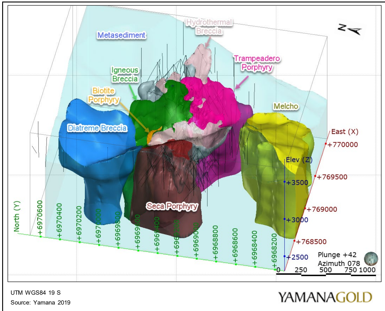
Figure 14-1: Lithology Model
