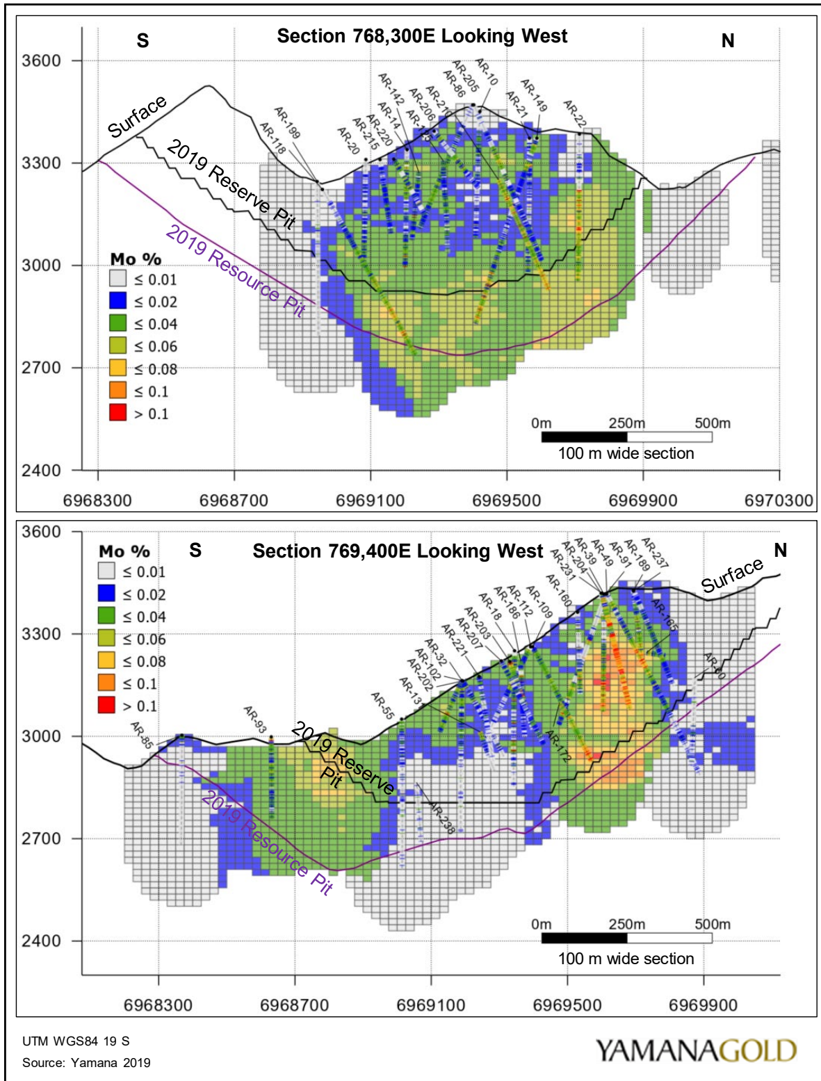
Figure 14-32: Estimated Molybdenum in Block Model and Drilling – Cross Sections
