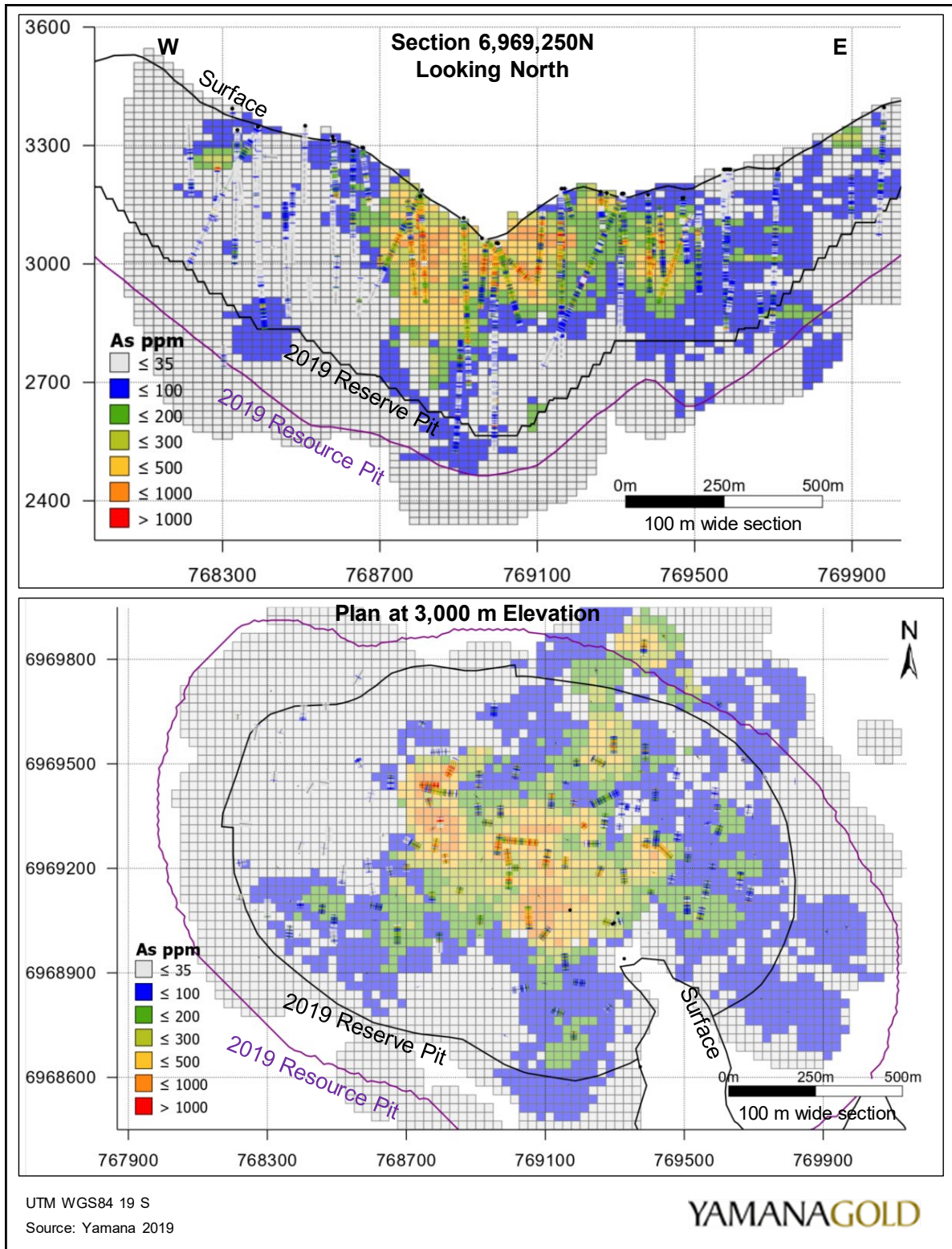
Figure 14-33: Estimated Arsenic in Block Model and Drilling – Cross Section and Plan View
