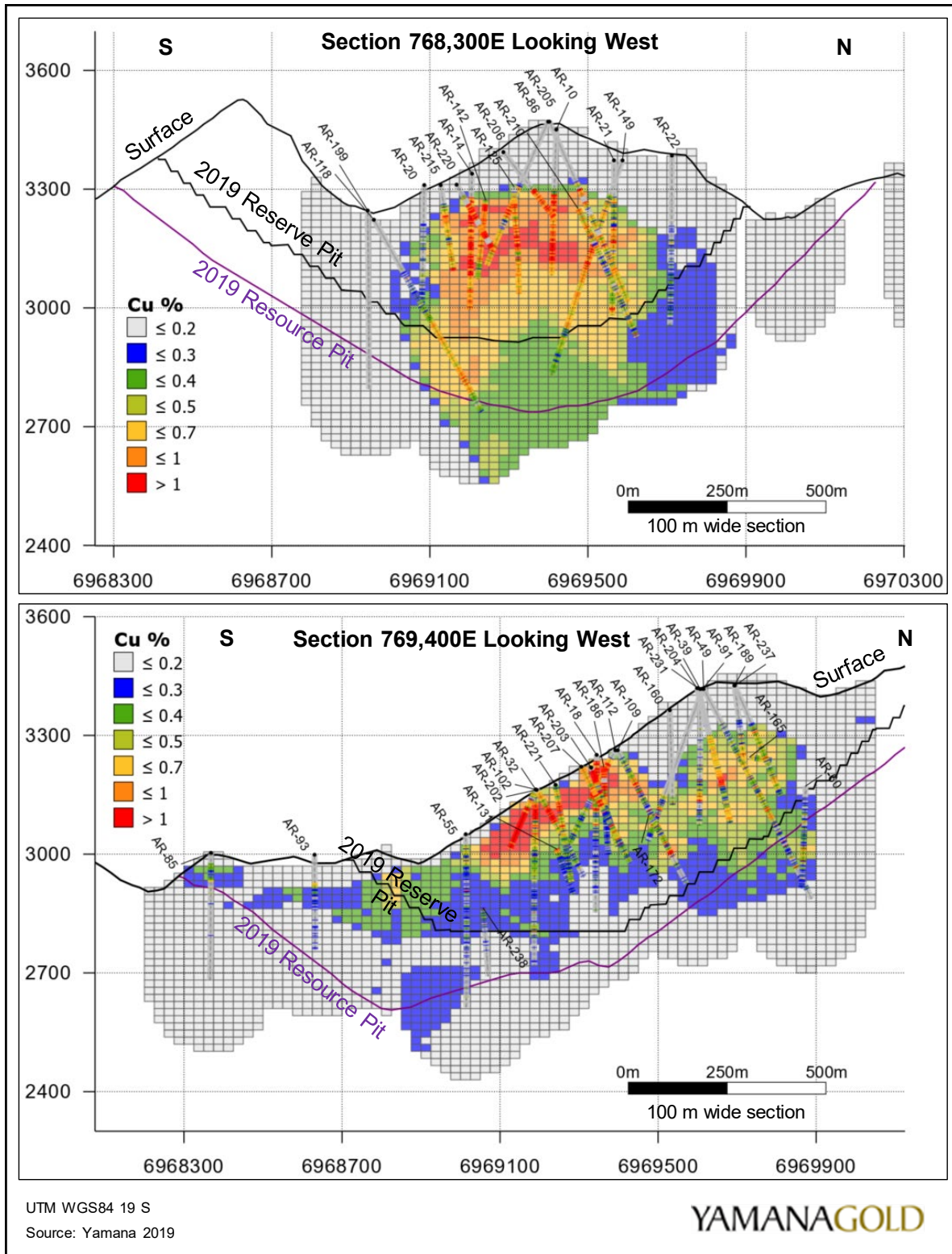
Figure 14-28: Estimated Copper in Block Model and Drilling – Cross Sections
