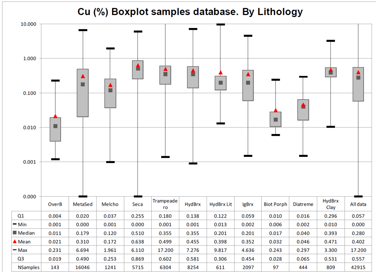
Figure 14-4: Descriptive Statistics and Box Plot for Copper by Lithology (Two Metre Sample Length)
