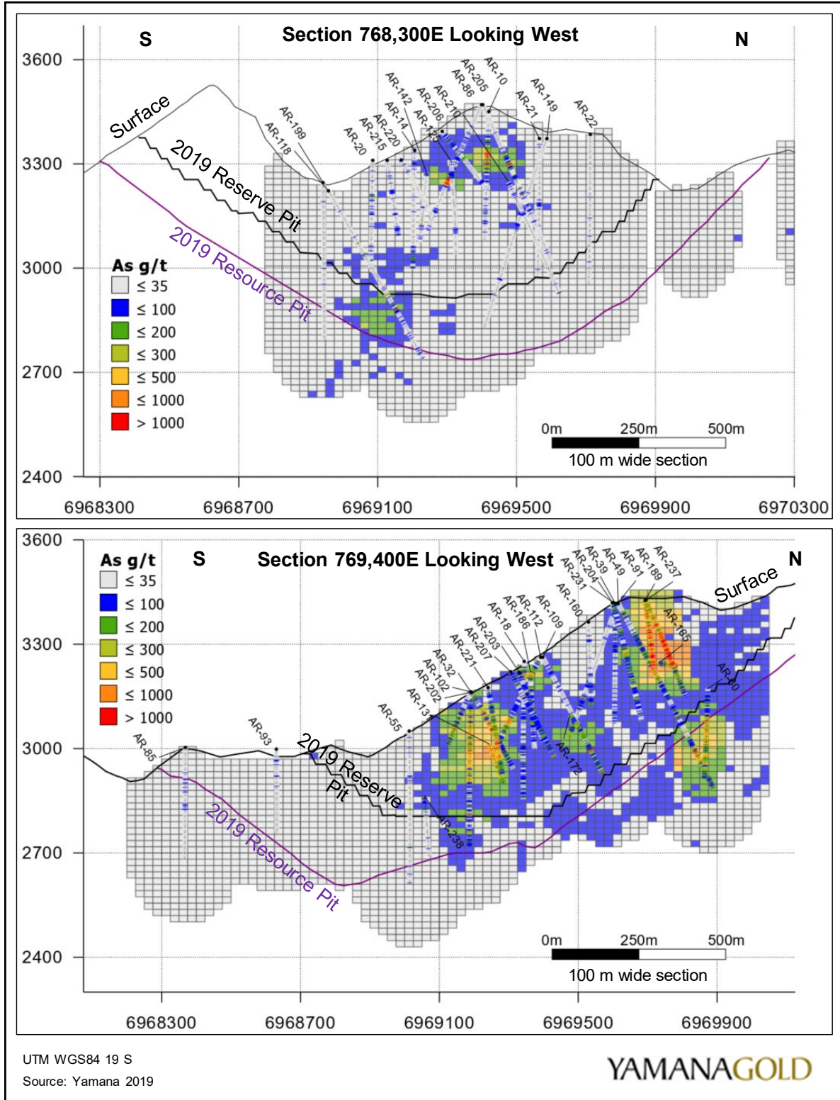
Figure 14-34: Estimated Arsenic in Block Model and Drilling – Cross Sections
