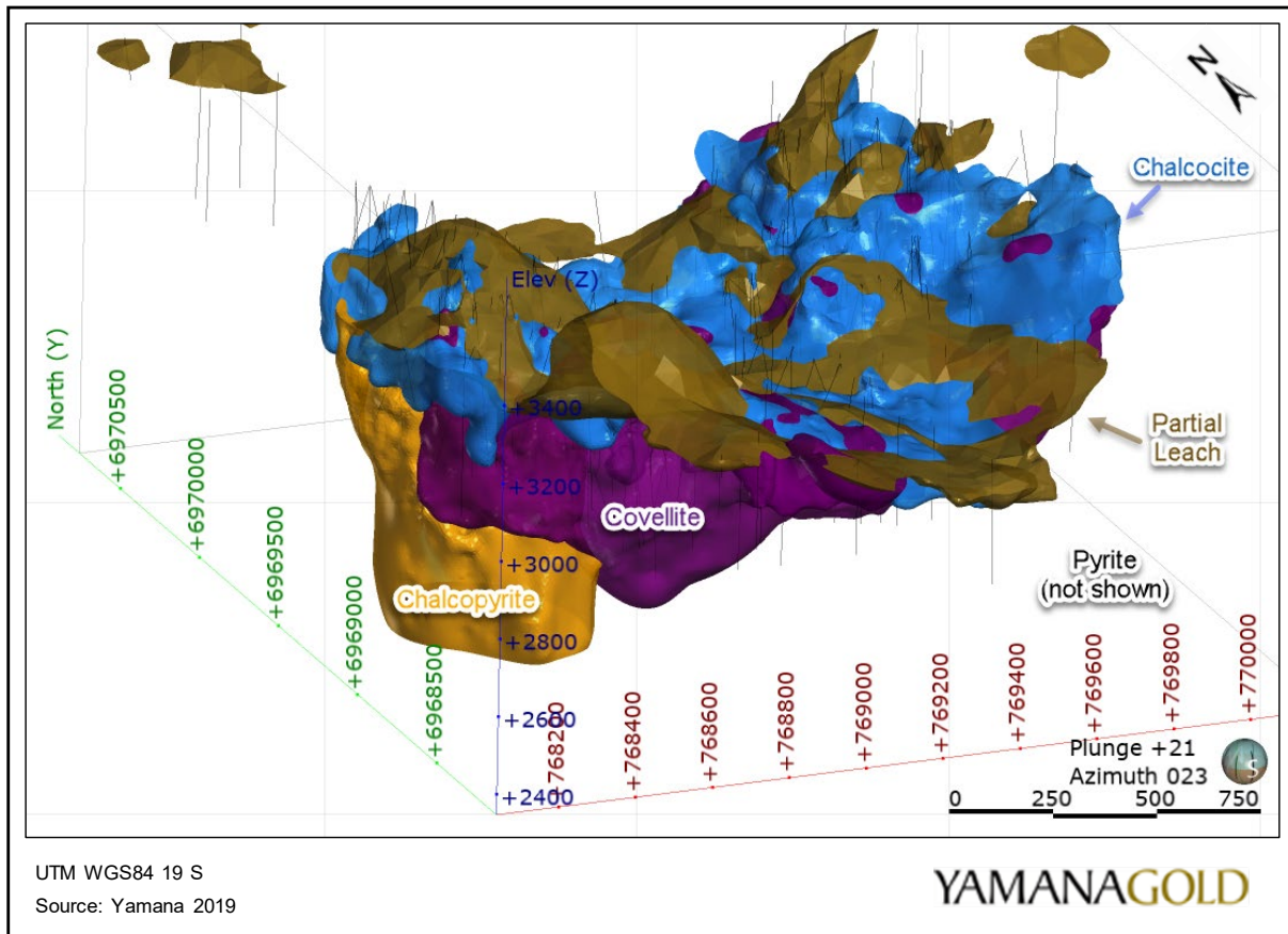
Figure 14-3: Mineralization Model
